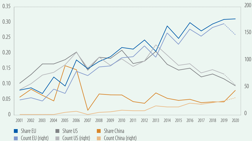
Figure E.3 Climate change mitigation technologies related to hydrogen (left axis: % of total patents; right axis: patent count), 2001-2020
