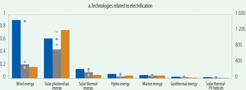
Figure E.2 Climate change mitigation technologies in electrification (left axis: % of total patents; right axis: patent count)
