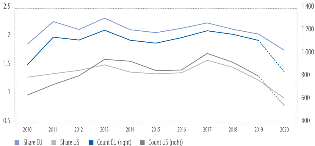
Figure 31 Green and digital patents in 2010-2020 (left axis: patent share in %; right axis: patent count), by region
