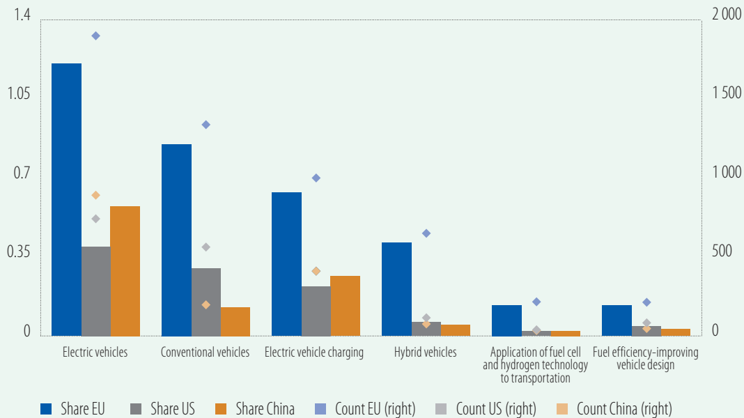
Figure E.1 Climate change mitigation technologies (left axis: % of total patents; right axis: patent count) related to transport and mobility, 2018-2020
