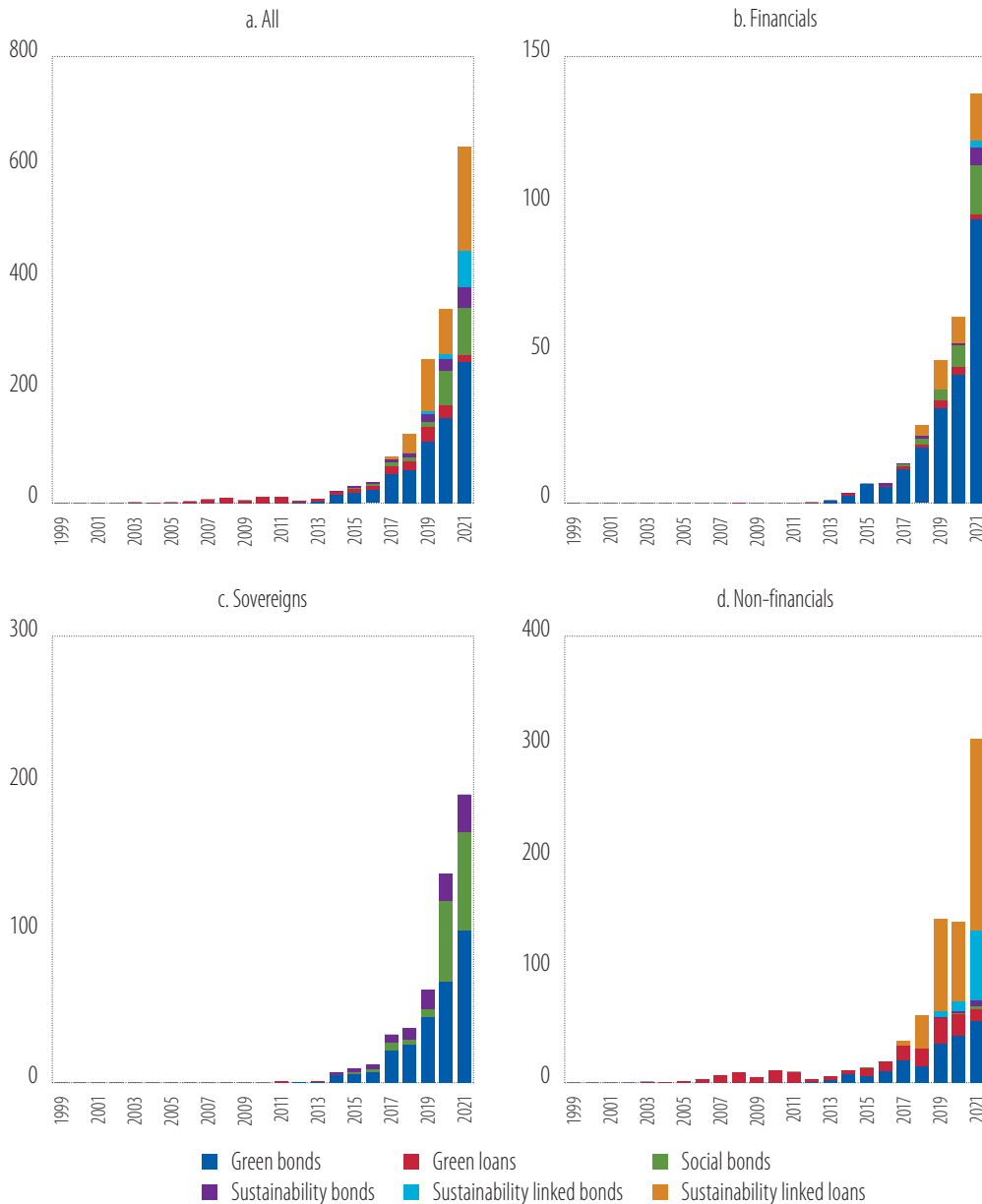
Figure 25 ESG debt issued by European entities (USD billion), by debt and issuer type
